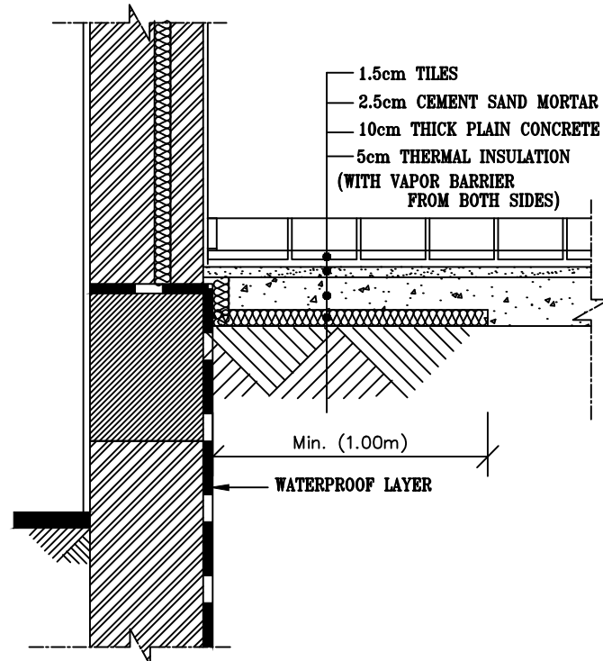
DETAIL ( 5A ) OF GROUND FLOOR
