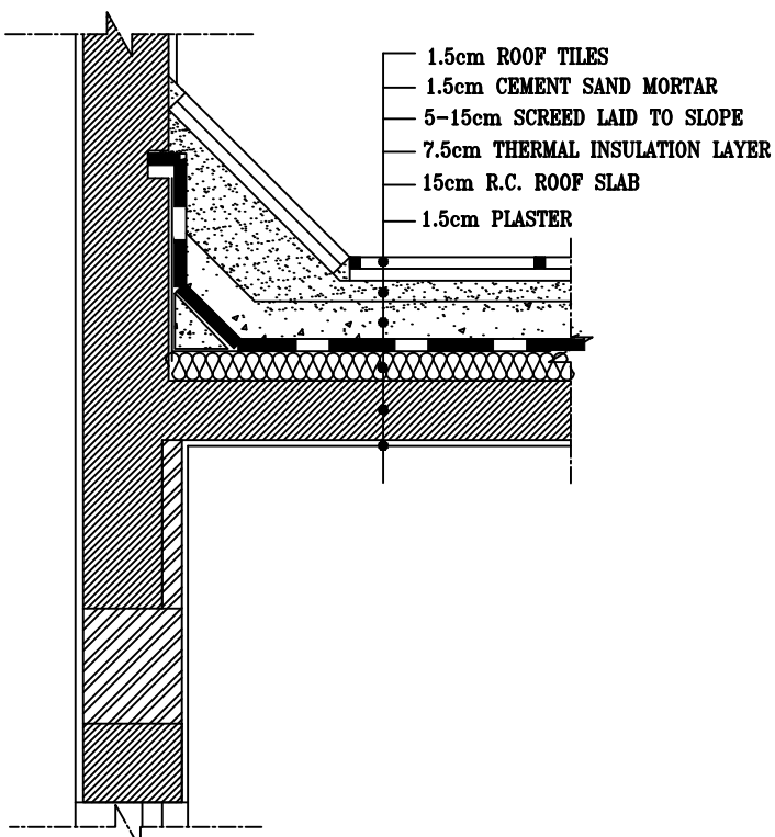
DETAIL ( 1C ) OF ROOF
