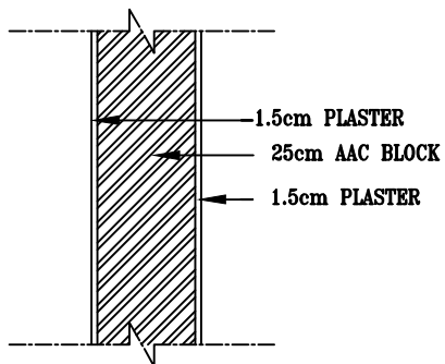
DETAIL ( 3C ) OF EXTERNAL COLUMN
