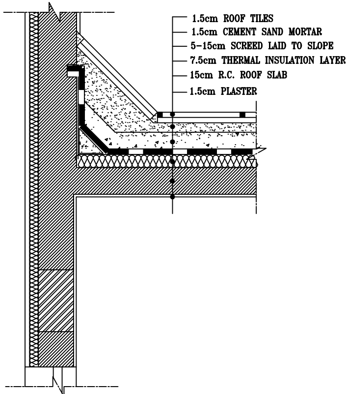
DETAIL ( 1B ) OF ROOF
