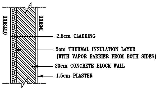
DETAIL ( 4B ) OF EXTERNAL WALL
