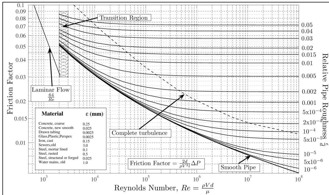
Figure 0-2— Moody Diagram for Estimation of Darcy-Weisbach Friction Factor
