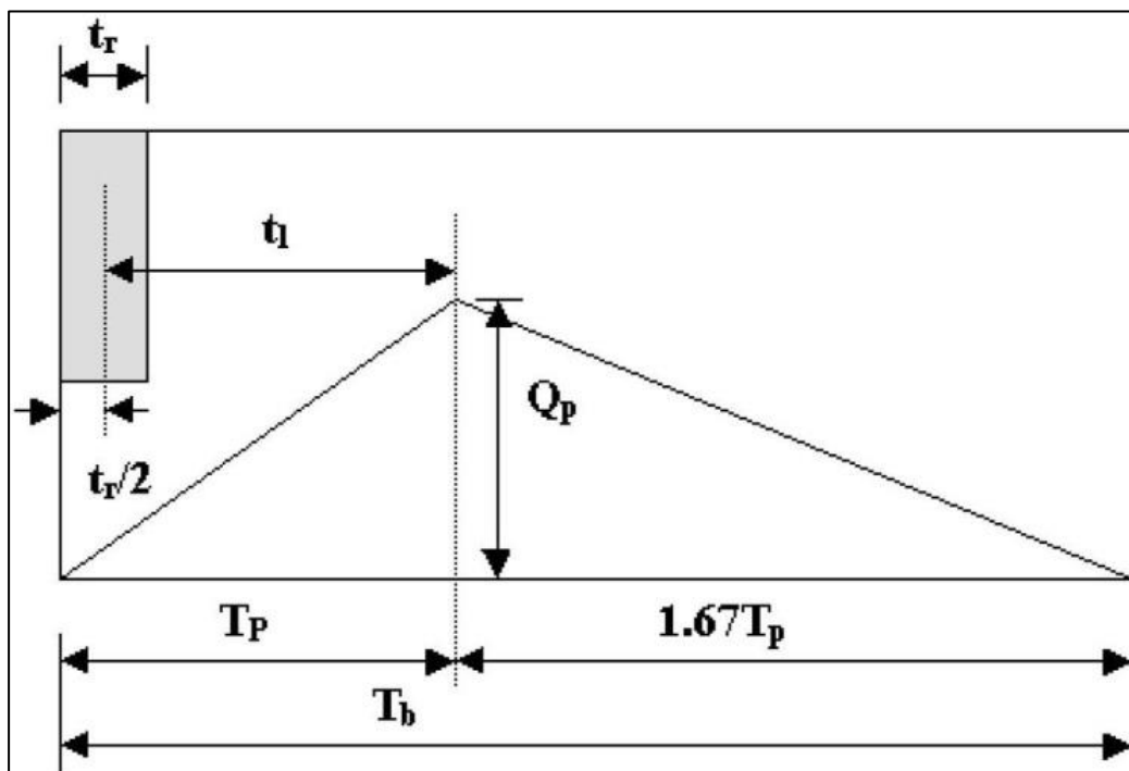
Figure 0-8— NRCS Dimensionless Unit Hydrograph
