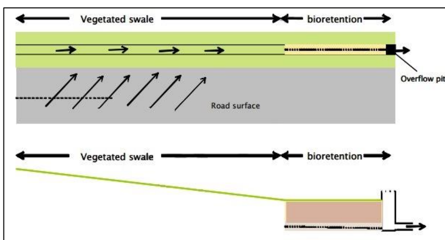
Figure 0-2— Conceptual Layout of Bio retention Swale (Gold Coast Planning Scheme Policy, 2007)
