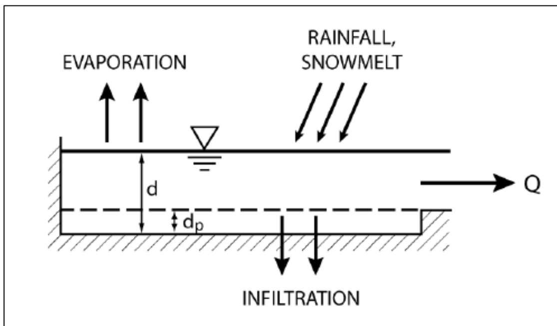
Figure 0-6—Non-Linear Reservoir (Innovyze, 2011)
